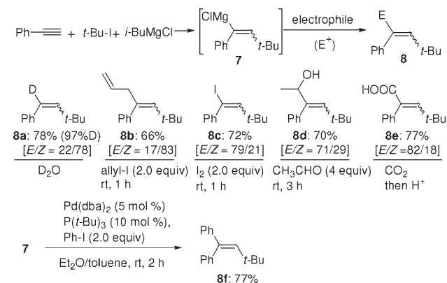
Scheme 2. Further Transformations of Vinyl Grignard Reagent 7
